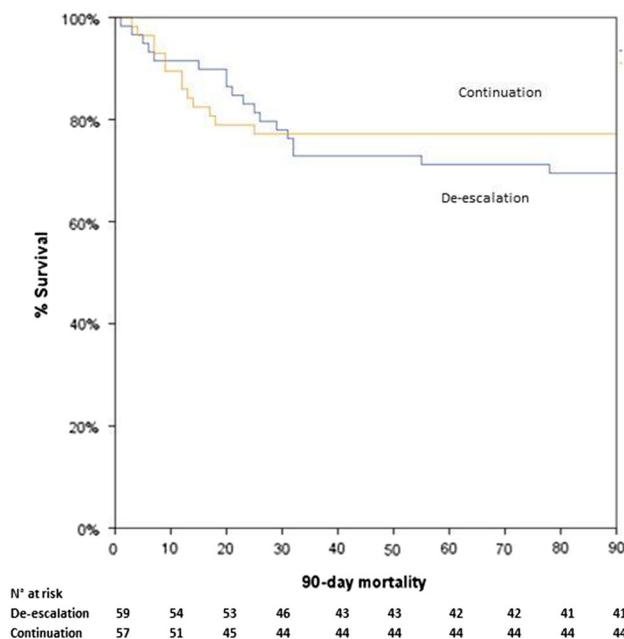
Fig. 2 Cumulative survival curves: no difference was observed in the groups
