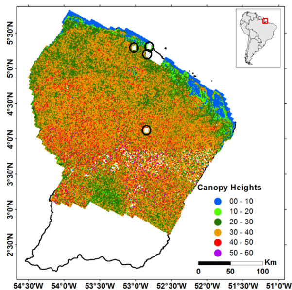
Figure 2. Map of canopy heights calculated from the airborne LiDAR LD dataset for French Guiana. The locations of airborne LiDAR HD datasets are delineated with circles.
