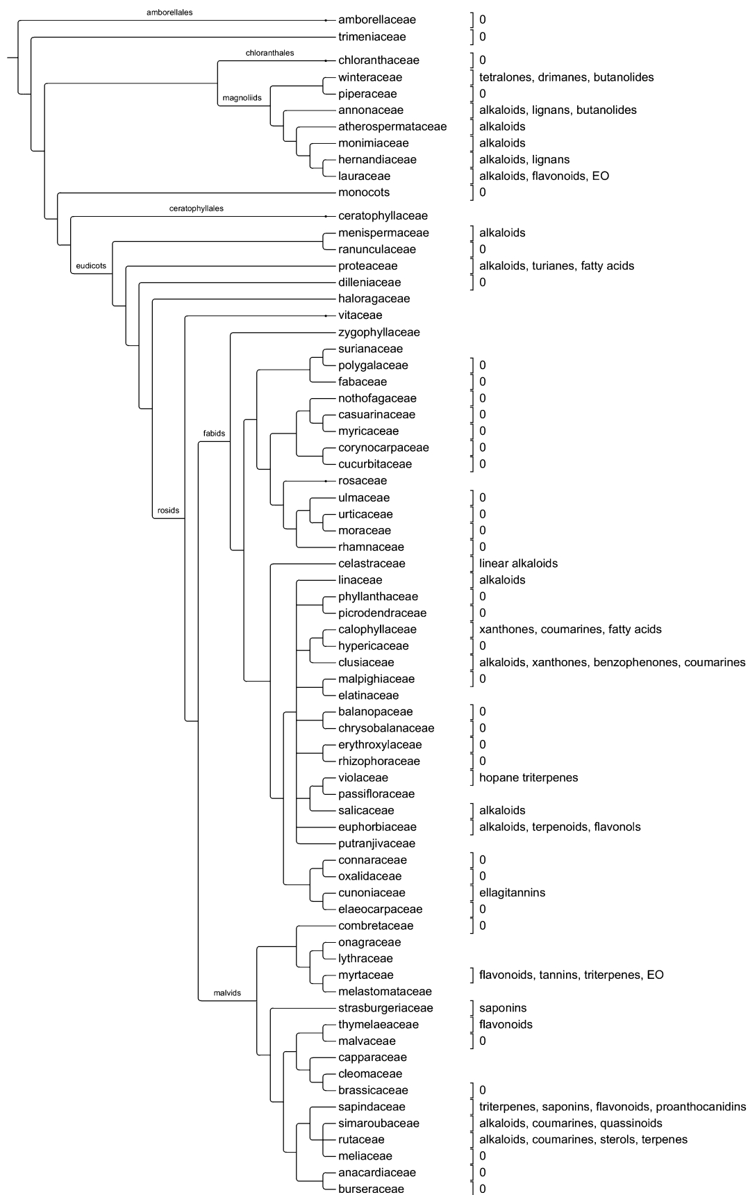
Fig. 1. Phylogenetic tree of New Caledonian basal angiosperms and eudicot rosids realized with TreeGraph and data from APGIII (see the Supporting Information 2 ) for the entire phylogenetic tree of New Caledonian plant families). Chemical families encountered in endemic species are mentioned on the right. EO, essential oil. 0 Corresponds to complete absence of chemical knowledge for any endemic species of a family (nothing is mentioned for families containing no endemic species).
