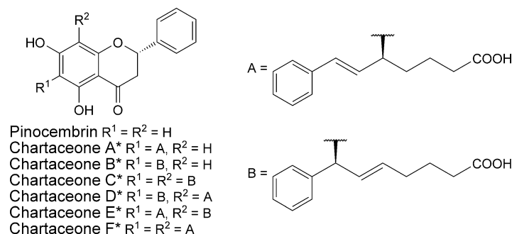
Fig. 8. Original flavonoids isolated from C. chartacea
