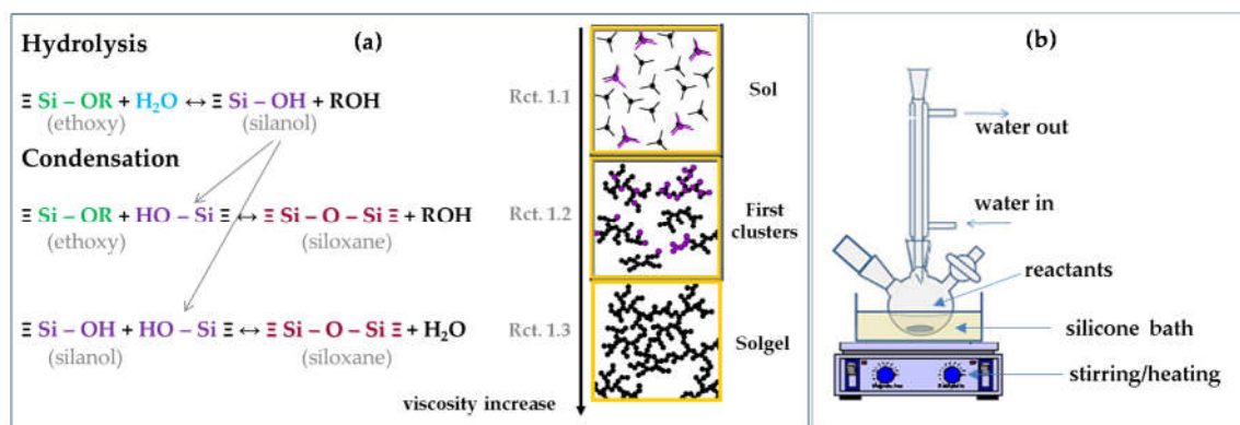
Figure 1. (a) Reactional mechanism of transformation of ETS40-based sol in solgel; (b) Experimental setup to run solgel synthesis. Rct. = reaction.
