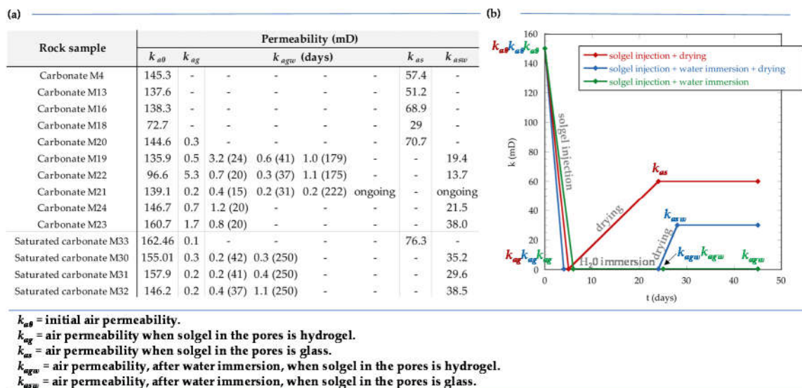
Figure 6. (a) Experimental results of the air permeability tests performed with vacuumed and water-saturated reefal carbonate samples; (b) scheme showing the experimental results presented in (a). k_{a0} indicates initial permeability before solgel injection; k_{ag} and k_{agw} denote permeability values measured when solgel inside the porous cores was hydrogel whereas k_{as} and k_{asw} show permeability values measured when solgel inside the porous cores was glass. k_{agw} and k_{asw} values correspond to the permeability measured in samples that were immersed in water before the permeability measurement. Note that the values in brackets shown in the Table indicate the number of days that the core sample was immersed in water before the permeability measurement.
