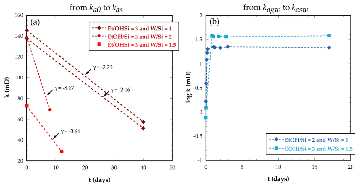
Figure 7. (a) Air permeability decrease as a function of the W/Si ratio; (b) Variation in air permeability during hydrogel drying for two hydrogel-filled cores immersed in water during 20 days. The values of the slope ( \gamma ) are indicated in Figure 7a.
