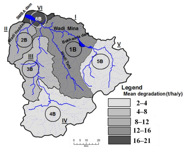
Figure 12. Specific degradation per sub-basin.
