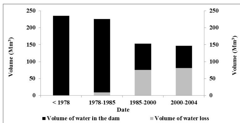
Figure 11. Evolution of the accumulated loss of water from the Sidi M'Hamed Benaouada Dam [14].
