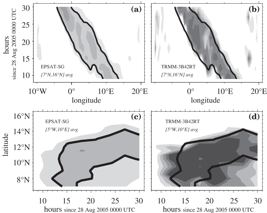
FIG. 5. (top) Longitude–time and (bottom) latitude–time diagrams of surface rainfall, averaged, respectively, over 7^{\circ} – 16^{\circ} N and 5^{\circ} W– 10^{\circ} E. Values above 1 mm are shaded, and darker as rainfall increases, from above 1, 2, 3, 4, 5, 10, 15, to 20 mm and above, for (left) EPSAT-SG and (right) TRMM-3B42RT. The black thick lines delineate the area where the EPSAT-SG rainfall estimate is greater than 2 mm. The y axis corresponds to the time at the end (the centered time) of the 3-h cumulative rainfall for EPSAT-SG (TRMM-3B42RT).
