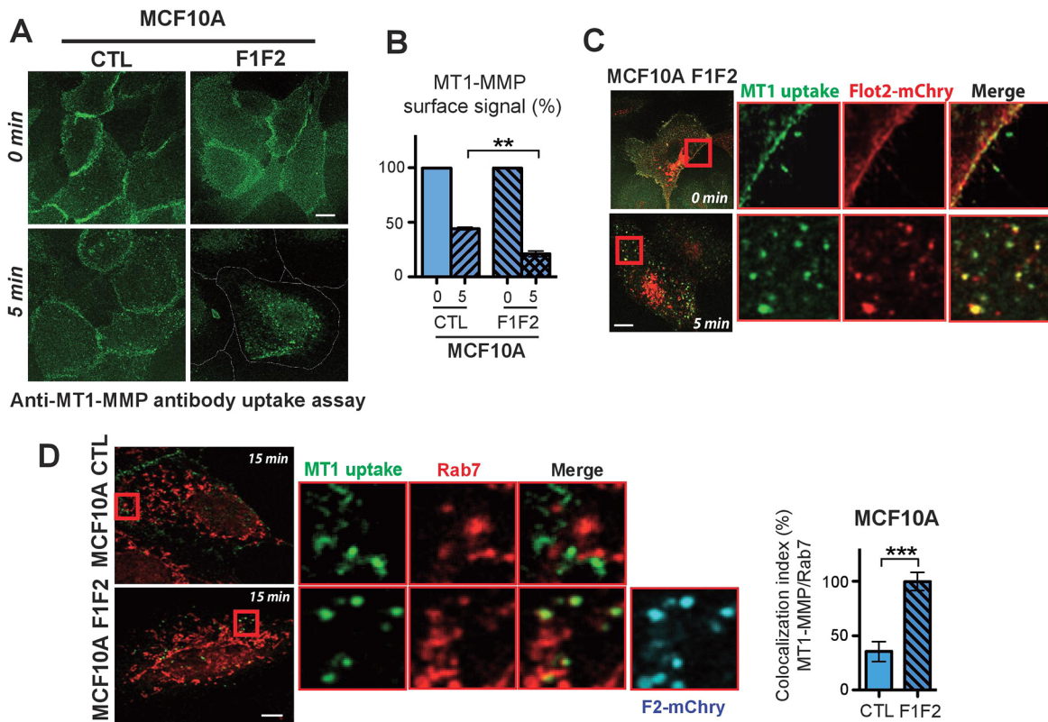
Fig. 6. Upregulated flotillins promote the formation of MT1-MMP-containing endocytic carriers and their movement to the endolysosomal compartment. (A,B) MCF10A CTL and F1F2 cells were incubated with an anti-MT1-MMP antibody at 4°C followed by incubation at 37°C for 5 min. Cells were fixed to allow MT1-MMP detection by immunocytochemistry (A) or by FACS (B) ( n=50,000 events per cell line). The histogram shows the mean \pm s.e.m. of five independent experiments. **P<0.01 (Student's t -test, two-tailed P -value). (C) Confocal micrographs of MCF10A F1F2 cells processed as in A showing flotillin-2 and MT1-MMP colocalization at the PM and in endocytic vesicles. (D) MCF10A CTL and F1F2 cells were processed as in A, fixed for 15 min after incubation at 37°C and incubated with anti-MT1-MMP and anti-RAB7 antibodies. Images are representative of at least five independent experiments. The histogram shows the mean \pm s.e.m. of four independent experiments ( n=20 cells). ***P<0.001 (Mann-Whitney test, two-tailed P -value). Scale bars: 5 \mu m.
