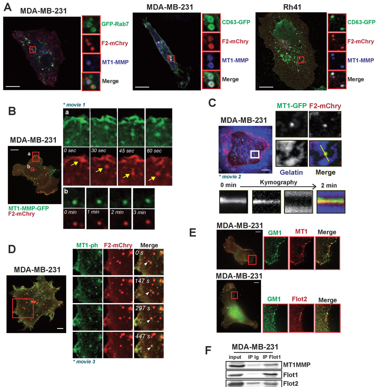
Fig. 3. Flotillins colocalize with MT1-MMP from the PM to the endolysosomal compartment. (A) Confocal micrographs of MDA-MB-231 and Rh41 cells transfected with FLOT2-mCherry (F2-mCherry) and GFP-tagged RAB7a or CD63 and incubated with an anti-MT1-MMP antibody to detect endogenous MT1-MMP. The zooms of boxed regions appear on the left side of each image. (B) Still images of a representative time-lapse series (see Movie 1) of one MDA-MB-231 cell that expresses MT1-MMP-GFP and F2-mCherry to show F2/MT1-MMP colocalization at the PM (a), at endocytic vesicles forming at the PM (a; arrow) and in intracellular vesicles (b). (C) Still images of one MDA-MB-231 cell that expresses MT1-MMP-GFP and F2-mCherry on Alexa Fluor 633-conjugated fluorescent gelatin (see Movie 2). Kymograph analysis shows the fluorescence intensities in a line scan through the boxed area. MT1-MMP and flotillin-2-containing vesicles are delivered at the degradation area. (D) Spinning disk images of a representative movie (Movie 3) of one MDA-MB-231 cell that expresses MT1-MMP-phluorin (MT1-ph) and F2-mCherry to visualize MT1-MMP exocytosis at F2-mCherry-positive vesicles (arrowhead). (E) GM1 molecules in MDA-MB-231 cells were labeled with Alexa Fluor 488-conjugated CTX-B subunit and then patched by addition of a secondary antibody. Endogenous MT1-MMP and flotillin-2 were labeled using specific antibodies. Merge images of GM1 and MT1-MMP or GM1 and flotillin-2 are shown. (F) Flotillin-1 was immunoprecipitated from MDA-MB-231 cell lysates. Co-immunoprecipitation of MT1-MMP and flotillin-2 was assessed by immunoblotting. Scale bars: 5 \mu m.
