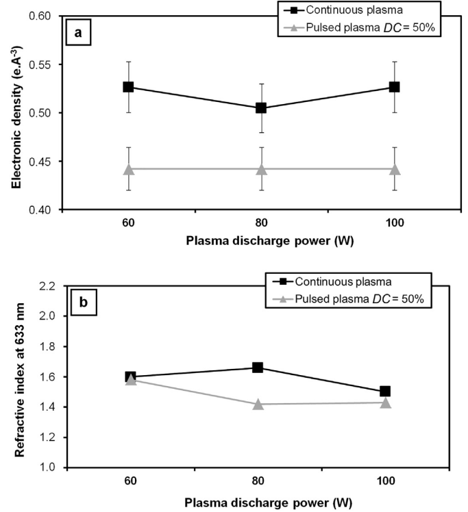
Fig. 4. Evolution of the film's (a) density as a function of the plasma deposition conditions ( \epsilon \sim 5\% ) (b) refractive index as a function of the plasma deposition conditions.
