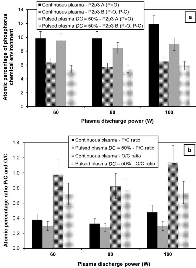
Fig. 8. Evolution of the film's atomic percentage (a) of the phosphorus chemical environments ( \epsilon \sim 10\% ) and (b) ratio P/C and O/C ( \epsilon \sim 20\% ) obtained from the atomic percentages obtained from XPS analysis as a function of the plasma deposition conditions.
