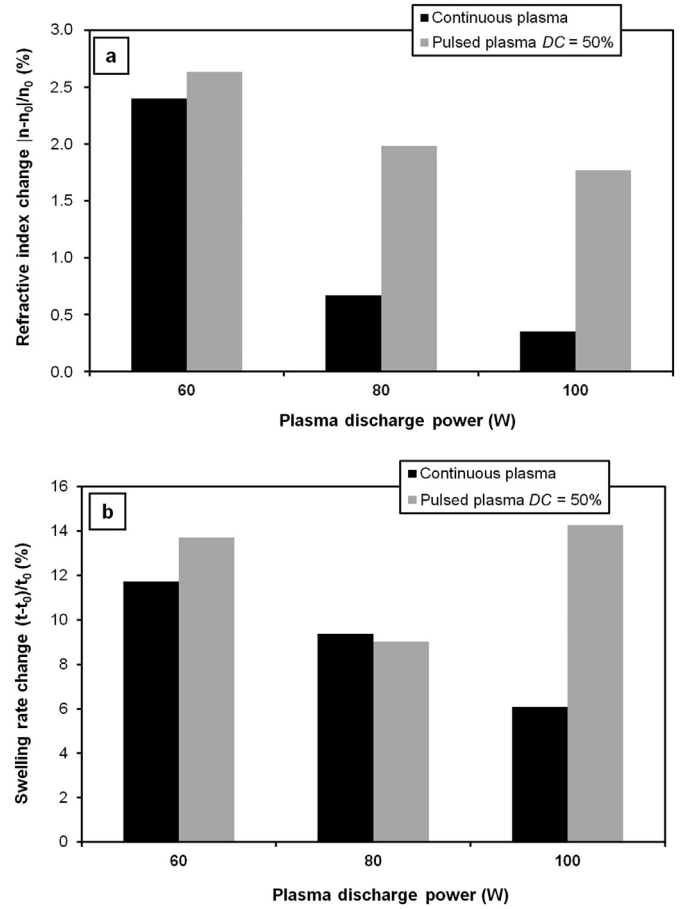
Fig. 10. Evolution of (a) the absolute value of the refractive index change |n - n_0|/n_0 (%) and (b) the swelling rate change (t - t_0)/t_0 (%) following water sorption of the plasma films.
