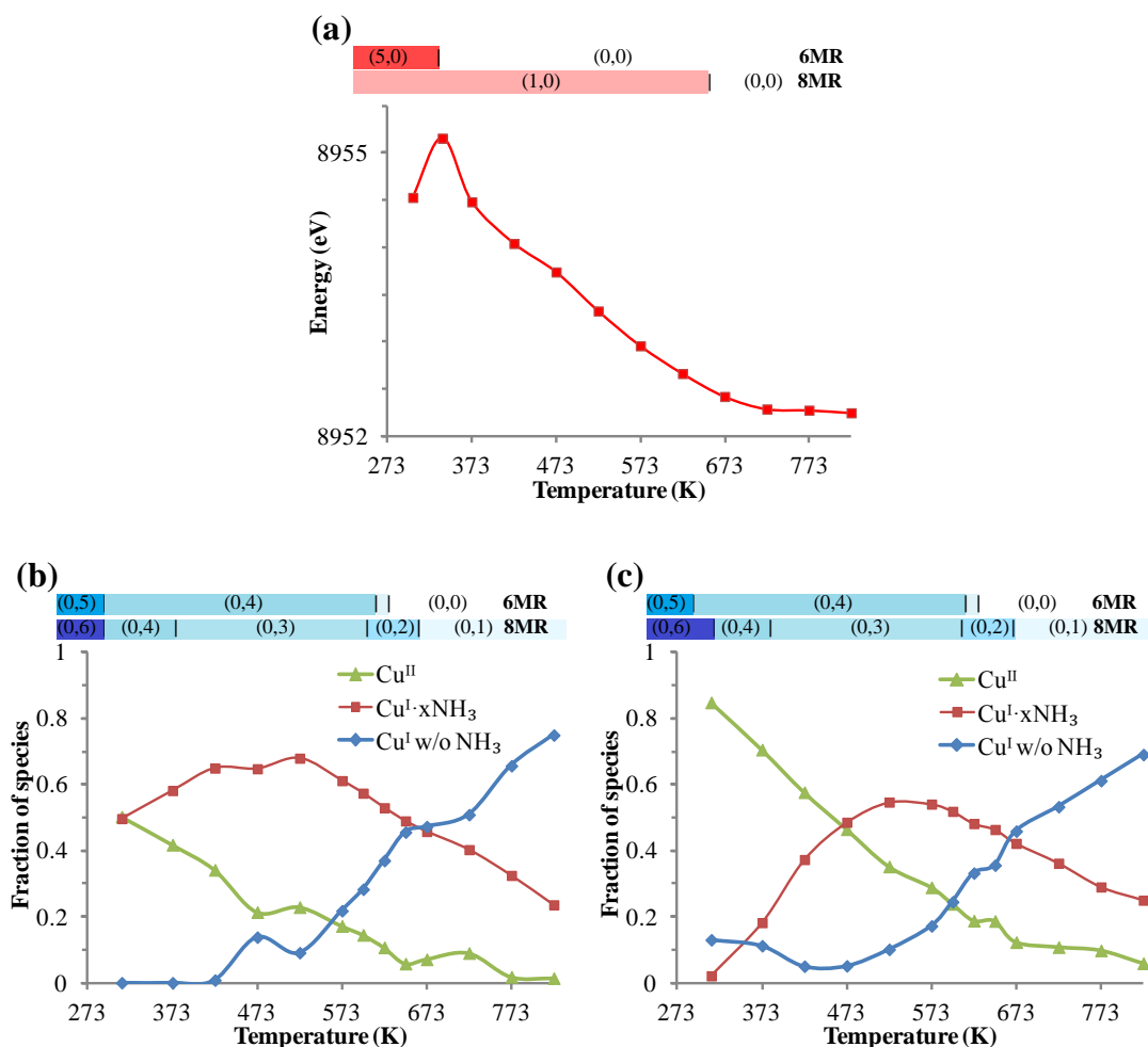
Figure 9. Results of LCA of XANES spectra at Cu K edge obtained during heating Cu-SSZ-13 zeolite in a flow of (a) He with P(\text{O}_2)= 10^{-2} bar and P(\text{H}_2\text{O})= 10^{-5} bar, (b) He with P(\text{NH}_3)= 10^{-3} bar, and (c) He with P(\text{NH}_3)= 10^{-3} bar and P(\text{H}_2\text{O})= 10^{-2} bar. Temperature ramp rate 10 K/min. Text lines on top of the graphs depict theoretical stability regions for Cu sites with \text{H}_2\text{O} and \text{NH}_3 ligands at 6MR and 8MR (derived from Figures 3, 4 and 7).
