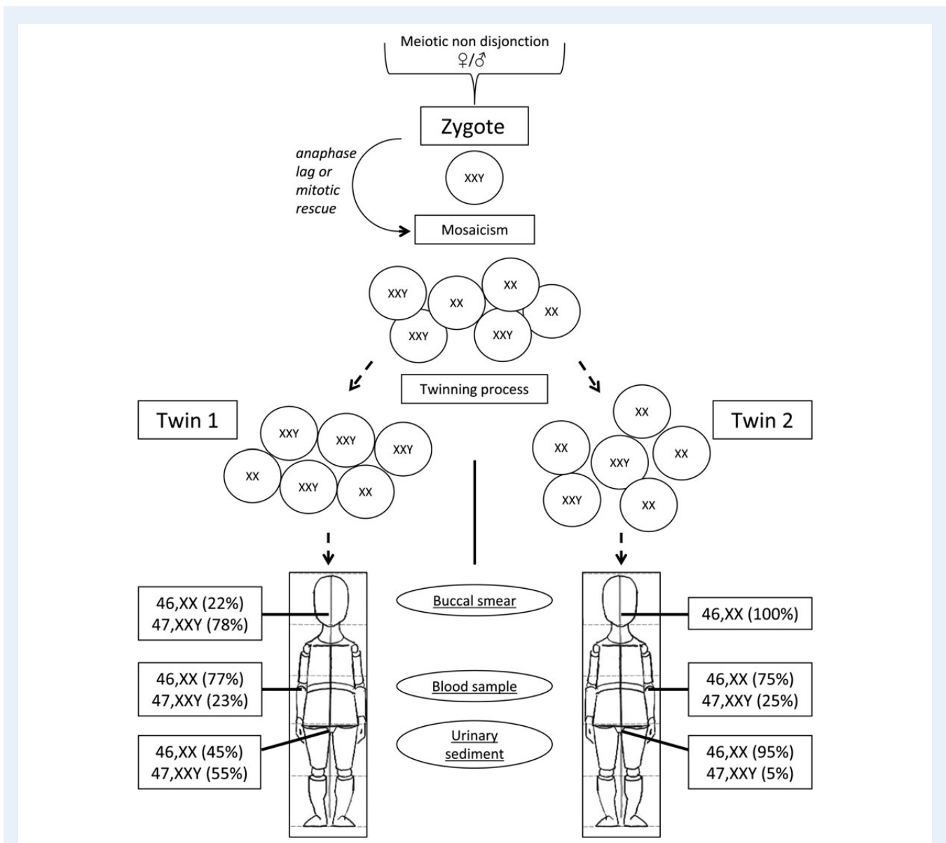
Figure 3 Schematic representation of the drift of the distribution of cell lines of the 47,XXY/46,XX mosaic in the twins during development.
