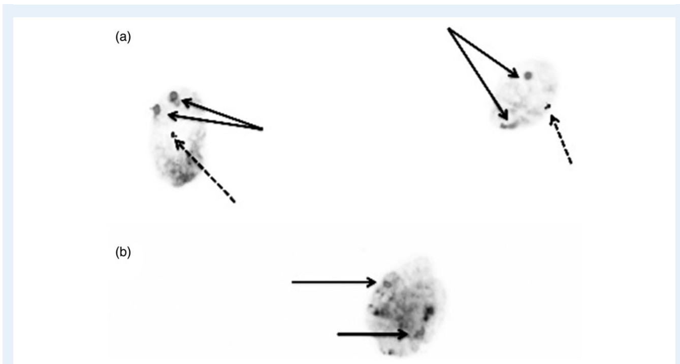
Figure 2 FISH results on the buccal smear sample of Twin 1 using Vysis probes. Full arrows point to DXZI (Xp11.1q11.1) and dotted arrows point to SRY. (a) Two XXXY nuclei. (b) One XX nucleus.
