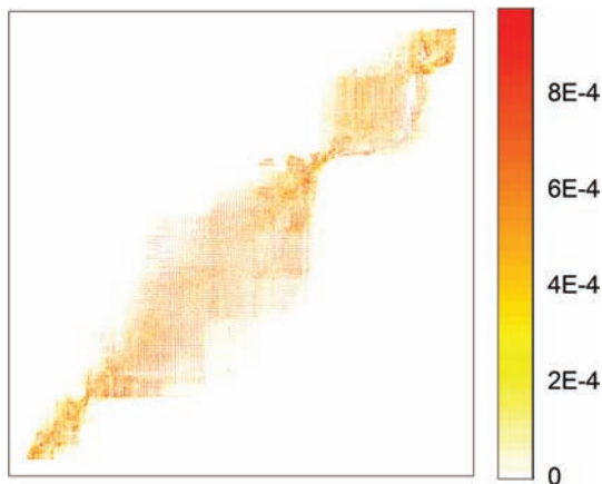
Figure 3. Connectivity matrix for the Mediterranean Sea. Colors represent probability of larval dispersal between the 770 sites.
