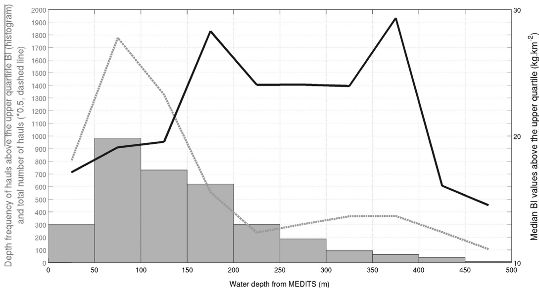
Fig. 5. Distribution by bottom depth (m, MEDITS data) of the upper quartile biomass index (i.e. above 8.4 kg km -2 ) of 0-group hakes (TL < 15 cm, histogram), total number of hauls (dash line) and median BI values above the upper quartile (solid line).
