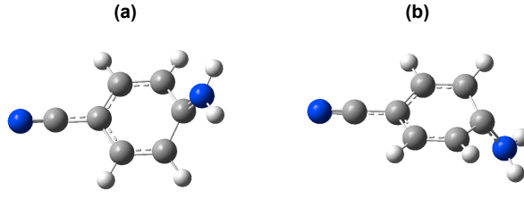
Fig. 4. Optimized geometry at the CASSCF(12,11)/cc-pVDZ level of theory of the pair of S_2/S_1 conical intersections denoted CI-C_S^+ (a) and CI-C_S^- (b).
