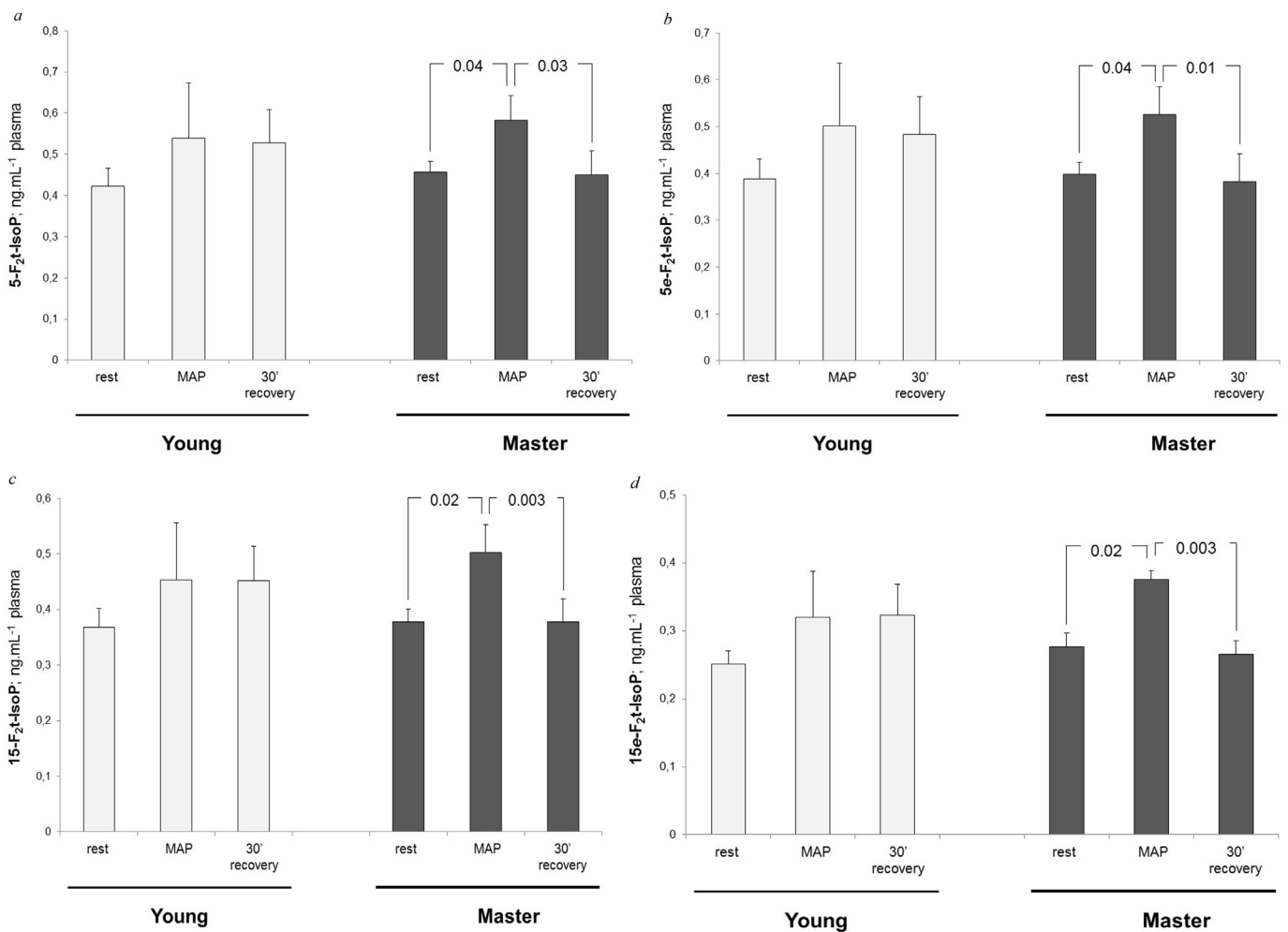
Fig. 1. Variation in F 2 -IsoP stereoisomer concentrations in plasma from rest to maximal aerobic power (MAP), and after 30-min of recovery in young and older (master) athletes. a . Variation in plasma 5-F 2 -IsoP concentrations. b . Variation in 5e-F 2 -IsoPs concentrations. c . Variation in 15-F 2 -IsoP concentrations. d . Variation in 15e-F 2 -IsoP concentrations.
