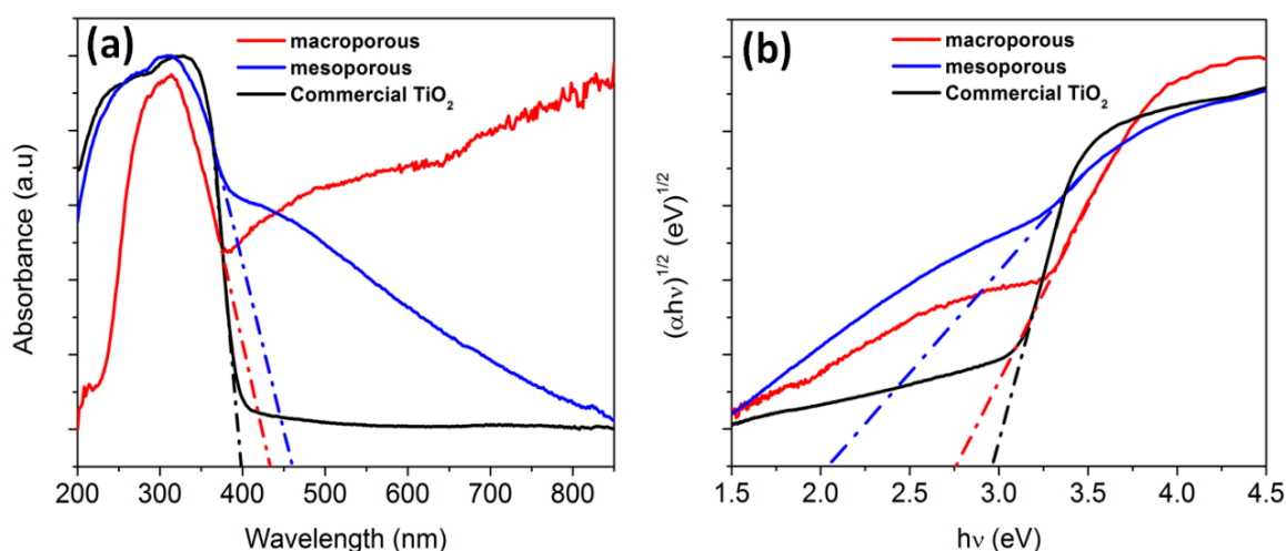
Figure 12. (a) UV-vis DRS spectra; (b) Tau plot: Namely (\alpha hv)^{1/2} vs. h\nu of macro/mesoporous nanocomposites and commercial \text{TiO}_2 .
