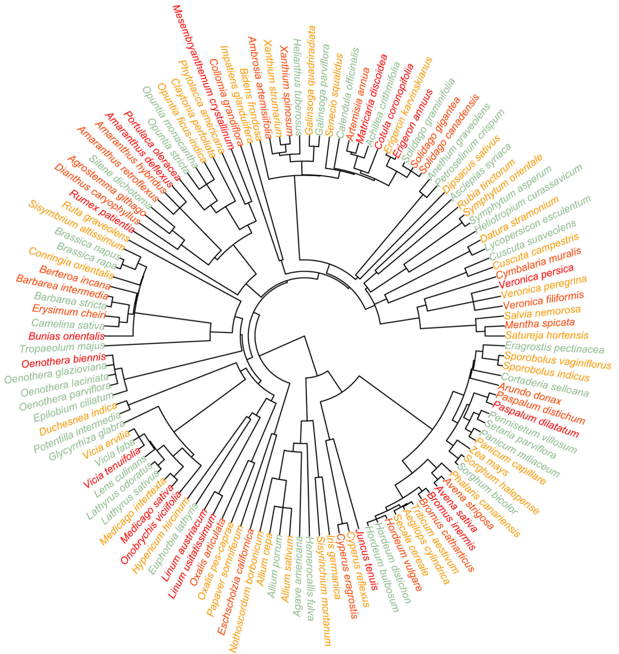
Figure 3. Phylogenetic tree of alien species in 50,000 French grassland plots with the corresponding commonness class. Color scheme follows the one in the contingency table in Fig. 1.
