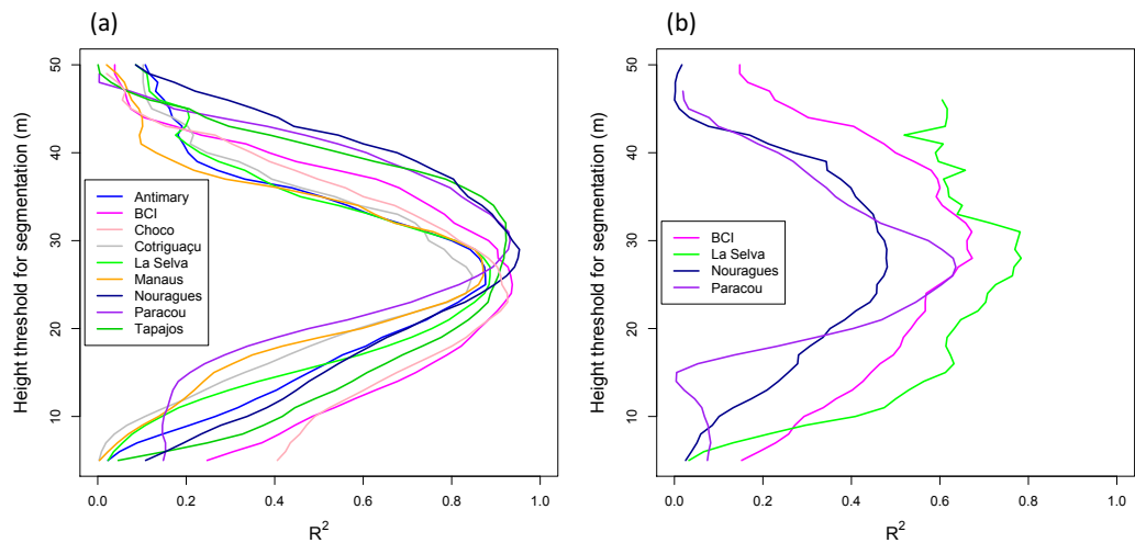
Figure 3. Distribution of R^2 between tree height thresholds used to determine LCA and \text{AGB}_{\text{Local}} in the nine 1 ha subareas (a) and distribution of R^2 between tree height thresholds and \text{AGB}_{\text{inv}} in 1 ha inventory plots of the four calibration sites (b). All optimal thresholds are between 23 and 30 m. The average maximal height threshold is 27 m.
