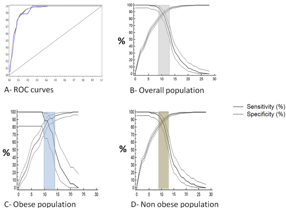
Fig 5. Bootstrapping analysis and the alternative approach. (A) ROC curves bootstrapped. Only the bootstrap of the ROC curve for the overall population is shown on this figure. (B–D) Determination of the alternative approach for the grey zone using the bootstrapping method: 9–12 for the overall population (B), 9.5–13 in the obese population (C) and 9–12 in the non-obese population (D).
