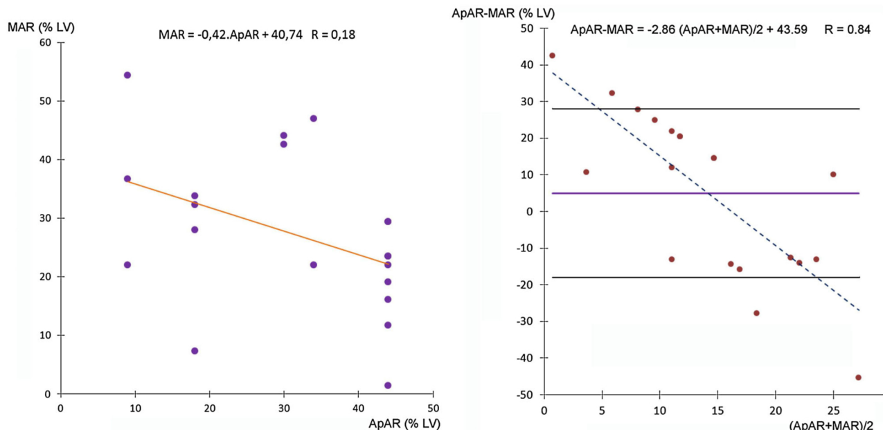
Figure 3. ^{123}\text{I} -MIBG defect area vs APPROACH-score for sub-occluded culprit artery (with MAR, ^{123}\text{I} -MIBG area at risk; ApAR, anatomical area at risk with modified APPROACH-score; LV, left ventricle). In the Bland-Altman analysis, the central purple continuous line represents the mean difference between the two techniques (ApAR and MAR) and the limits of agreement are given by the mean difference \pm 2 standard deviations of the difference ( black lines ). The dotted line represents the linear regression line between the difference and the arithmetic mean of the two measures.
