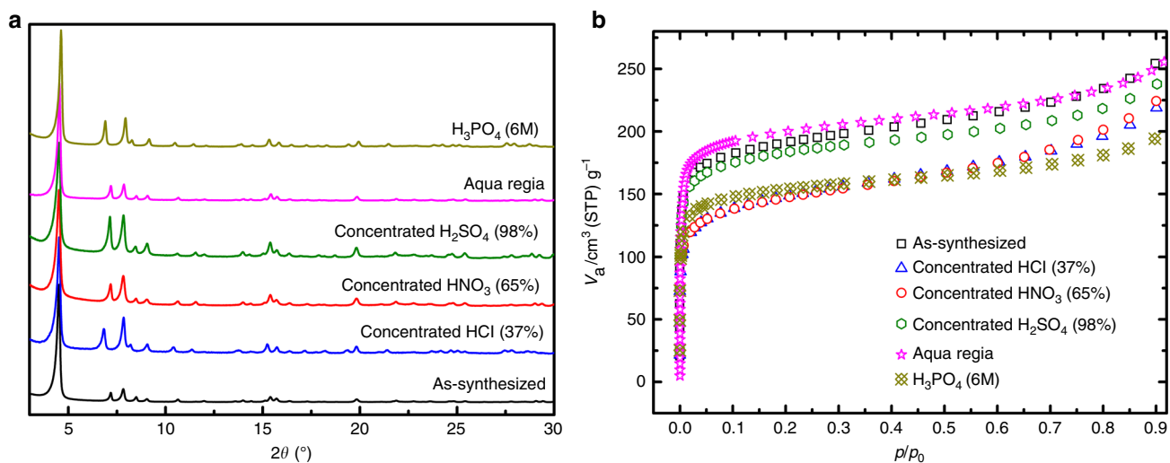
Fig. 3 Chemical stability test results of MIL-177-LT. a PXRD patterns and b nitrogen adsorption isotherms of MIL-177-LT samples before and after chemical treatment in various acids
