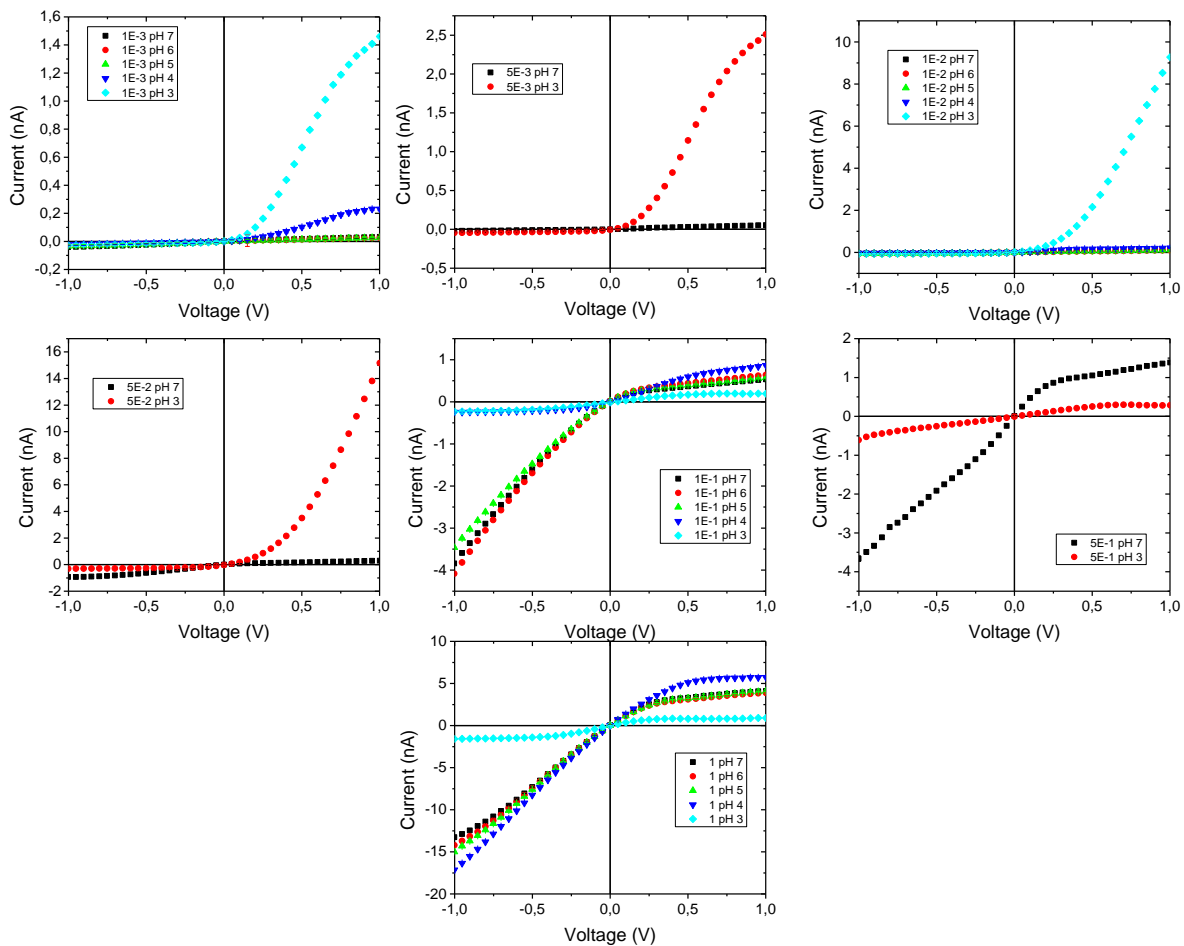
Figure SI-2 : I-V dependence of nanopore (d=98 nm) functionalized with PEI/PAA 10 bilayers
