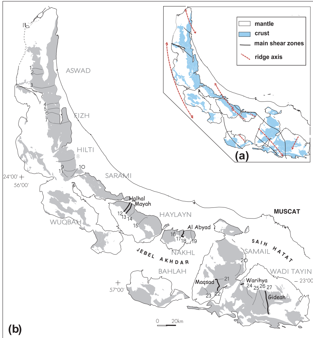
Fig. 1. (a) Simplified map of the Oman–UAE ophiolite including the inferred location of the palaeo-ridge axes and main shear zones [modified from Nicolas et al. (2000)]. (b) Simplified map of the Samail ophiolite. Thin numbered lines represent the log-sections of Fig. 4, along wadis where alteration facies have been studied. Bold lines are the wadi sections selected for detailed petrological and geochemical work in this study.
