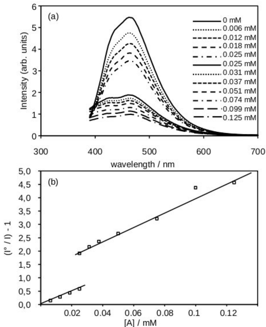
Figure 5. (a) Emission spectra ( \lambda_{\text{excit}} = 375 nm) and (b) Stern-Volmer plot for sample of PMHS containing 1 immersed in chloroform solution with increasing concentration of picric acid (a period of 1 h passed between the two measurements in the presence of 0.025 mM picric acid).
