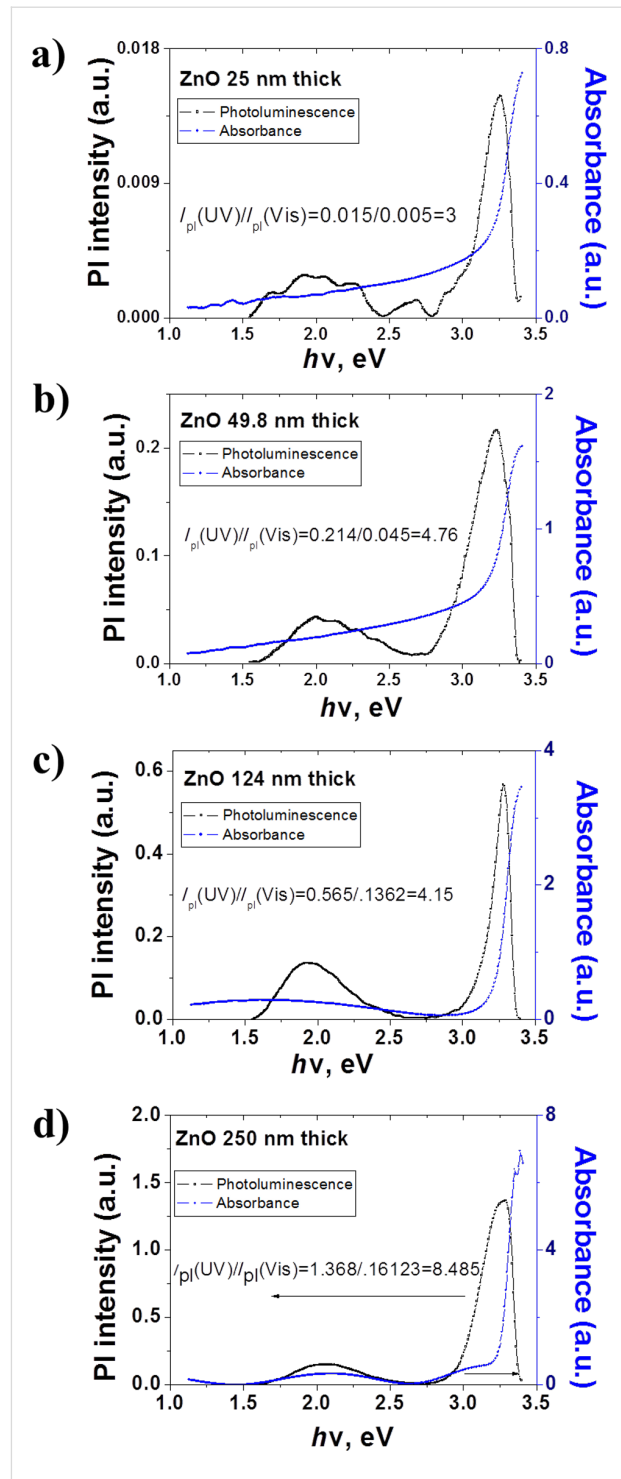
Figure 4: PL and absorption spectra of 25 (a), 49.8 (b), 124 (c), and 250 nm (d) thick ZnO ALD films.
