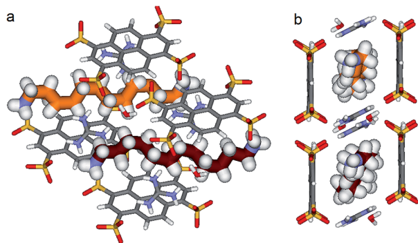
Fig. 7 X-ray structure of \text{PTSG}\{3\} : (a) Side and (b) Front view of the \text{PTSG}\{3\} inclusion complex. 1,12-diammoniumdodecane, 3 presents inside the \text{PTSG} box, two highly compressed architectures 3a and 3b having 6 gauche (orange) and having 4 gauche (red-violet) conformations, respectively.
