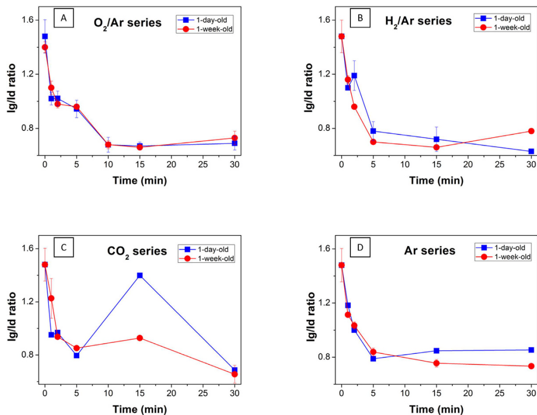
Figure 3. Raman I_g/I_d ratio of the O_2/Ar series (A), H_2/Ar (B), CO_2 (C) and Ar (D).
