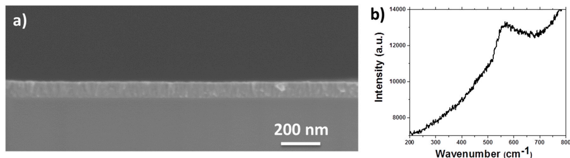
Figure 4. (a) SEM cross section image of \text{TiO}_2 films deposited by ALD on Si substrates and (b) Raman spectrum of \text{TiO}_2 films deposited by ALD.
