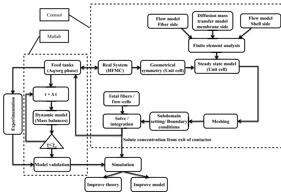
Fig. 3. Model algorithm/numerical scheme.
